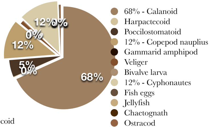
Cowlitz Bay Jan 16, 2008
